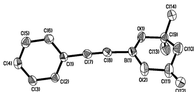
Figure 7. ORTEP diagram of 17 . Selected bond distances [Å] and angles [°]: C(7)–C(8) 1.205(5), C(8)–B(1) 1.541(6), B(1)–O(1) 1.339(5), B(1)–O(2) 1.364(5); O(1)–B(1)–O(2) 124.3(4).
