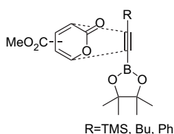
Figure 3. Cycloaddition regiochemistry.
