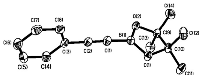
Figure 6. ORTEP diagram of 5c . Selected bond distances [Å] and angles [°]: C(1)–C(2) 1.201(3), C(1)–B(1) 1.535(3), B(1)–O(1) 1.358(2), B(1)–O(2) 1.362(2); O(1)–B(1)–O(2) 114.84(17).
