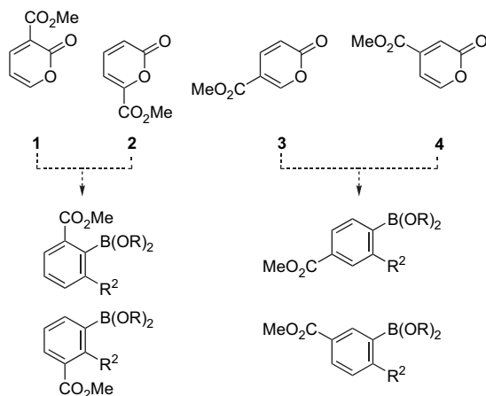
Figure 2. Cycloadditions of isomeric 2-pyrones.
